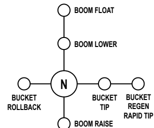
JOYSTICK HANDLE OPERATION LOOKING AT HANDLE KNOB
