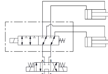
TYPICAL APPLICATION
