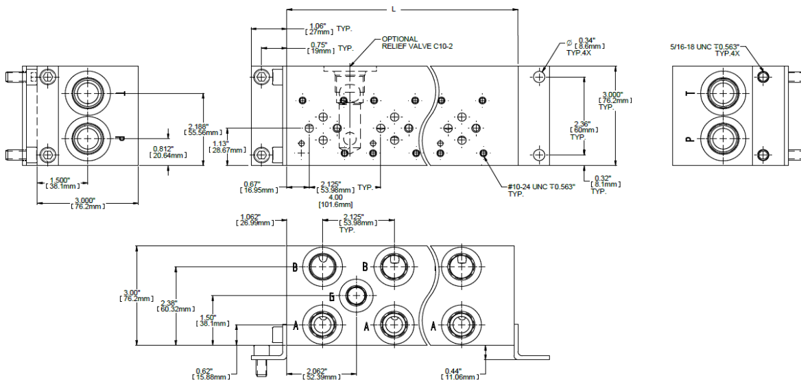
PARALLEL CIRCUIT WITH OPTIONAL RELIEF VALVE SHOWN
