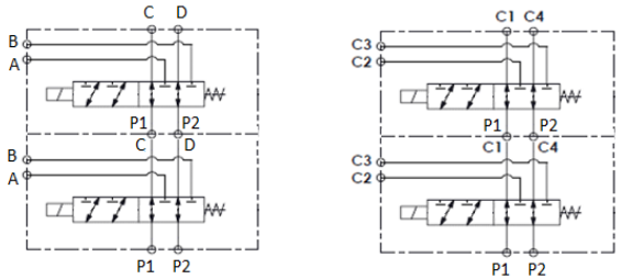
MOP & SVK MODELS 8 WAYS SHOWN
