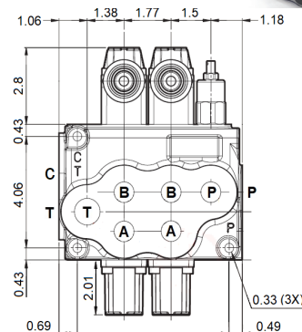
FITS "SD11" WALVOIL FOOTPRINT
